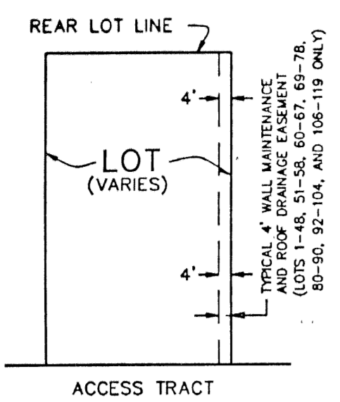
TYPICAL LOT DETAIL NOT TO SCALE 4' WALL MAINTENANCE AND ROOF DRAINAGE EASEMENT (SEE DEDICATION NO. 6)
